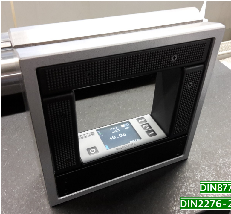
MICROLEVEL: modern electronic with approved precision from Roeckle
